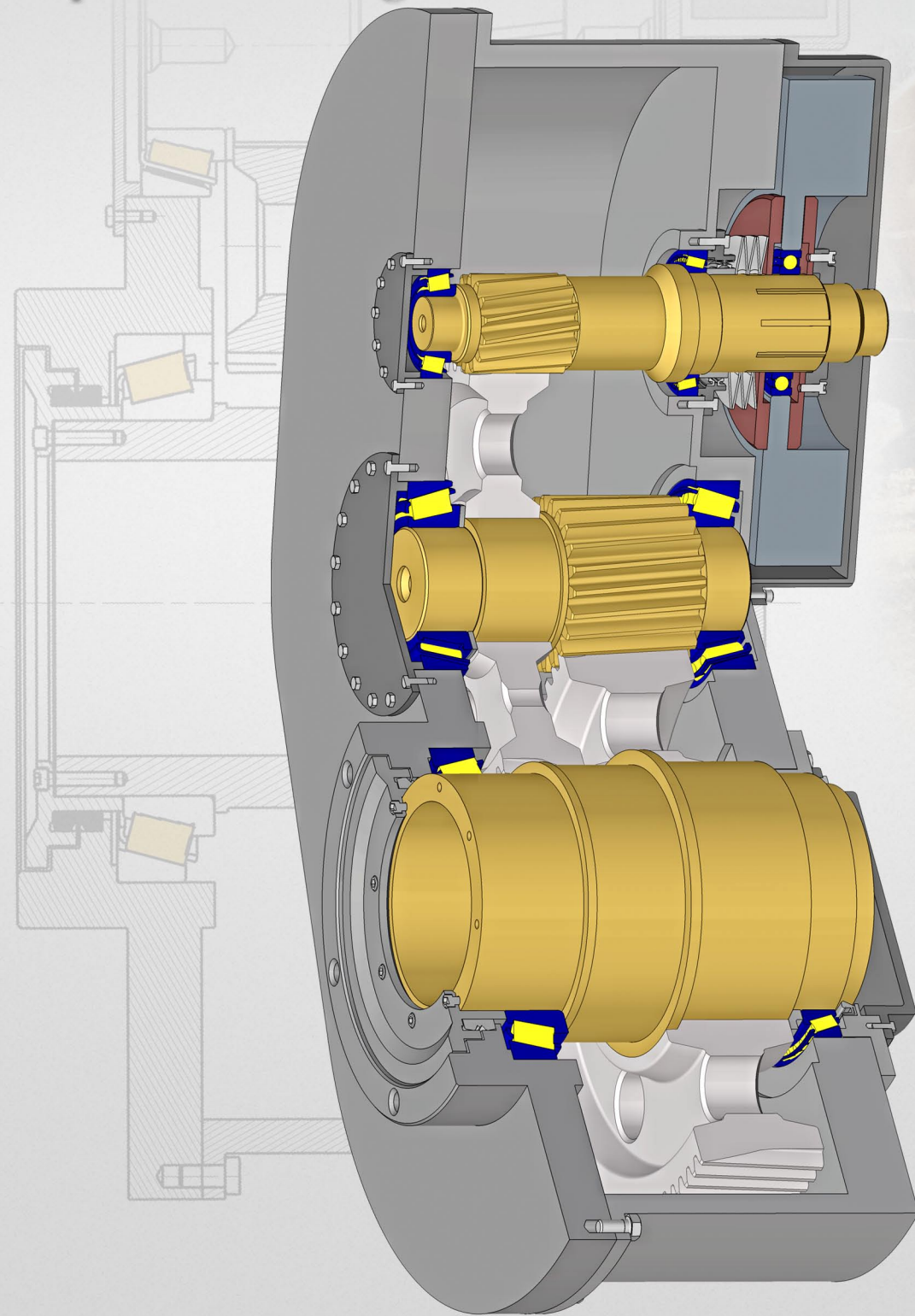
Project 'E.M. Gear' Trencher flywheel gearbox
