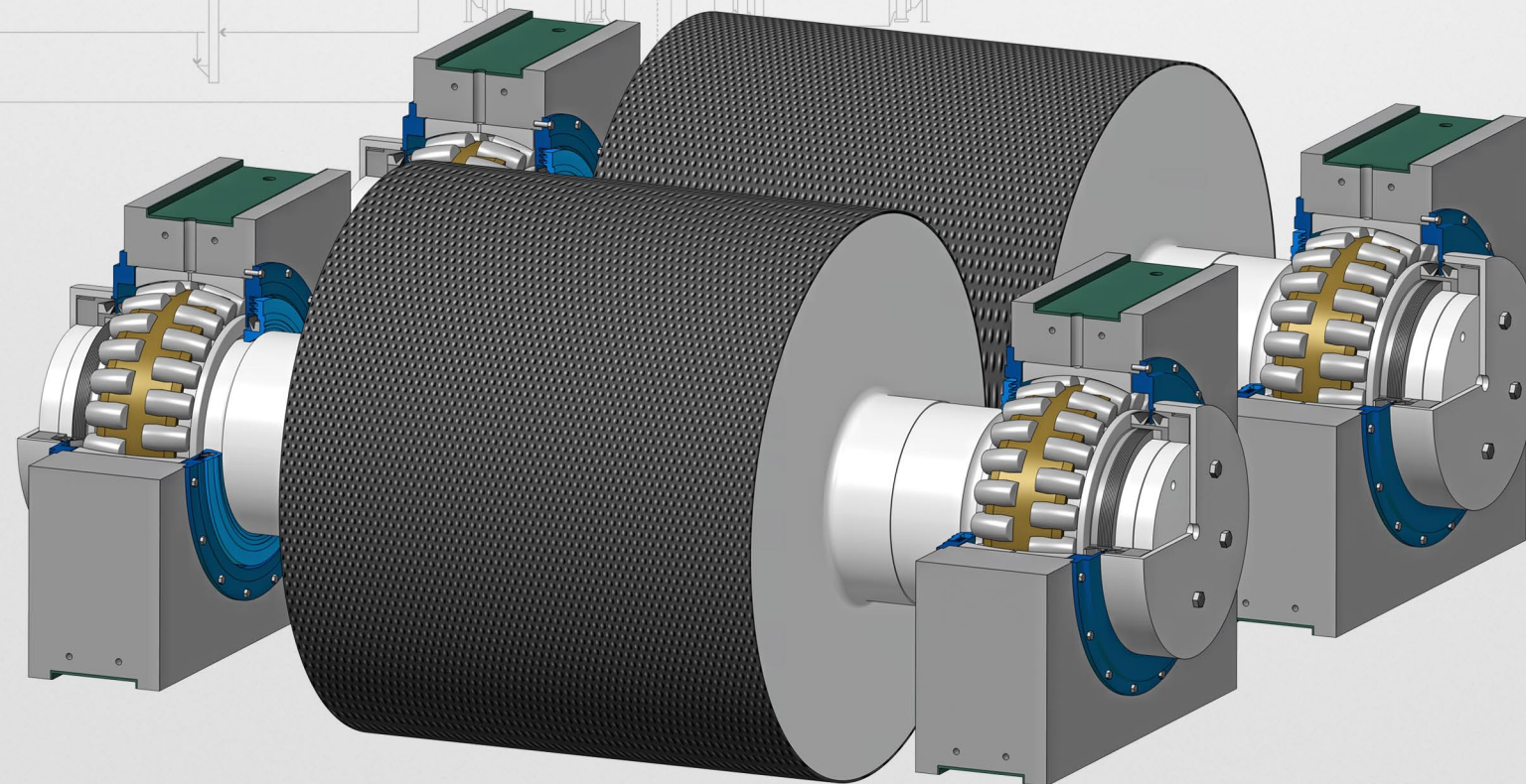
Project 'H.M. 1' Horizontal mill press rolls
